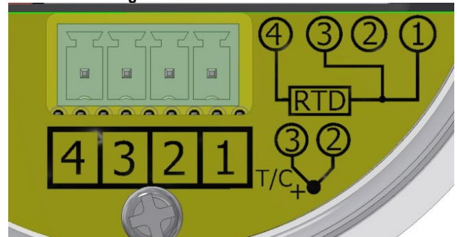
Figure 3: Connection diagram
