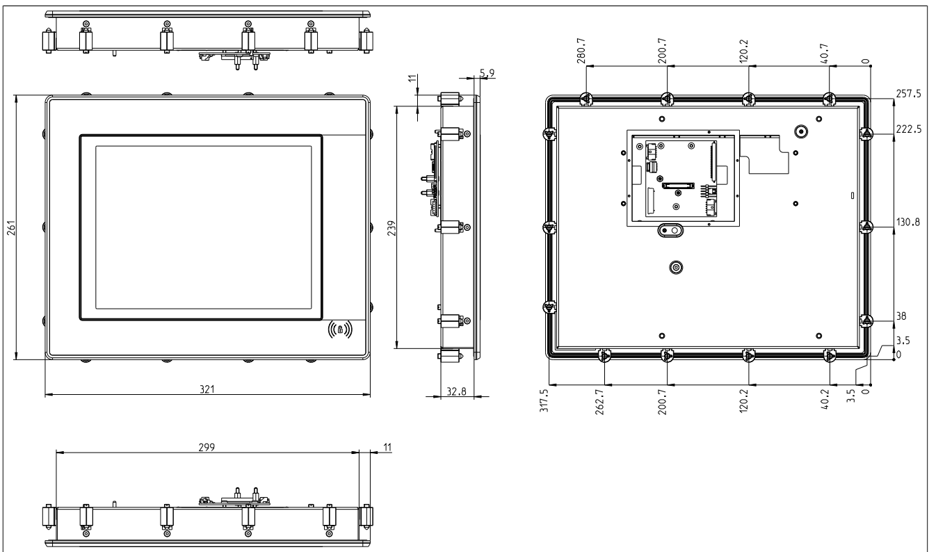
Figure 9: 5AP1125.1044-I00 - Dimensions
