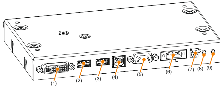
Figure 4: Overview of interfaces - SDL/DVI receiver link module
