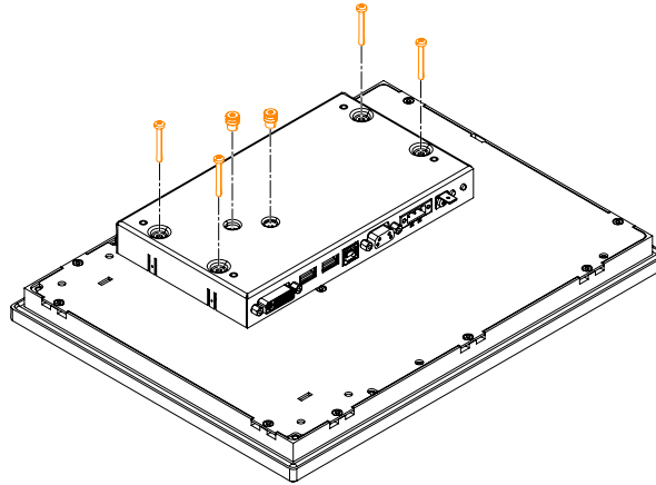
Figure 11: Removing the Torx screws
