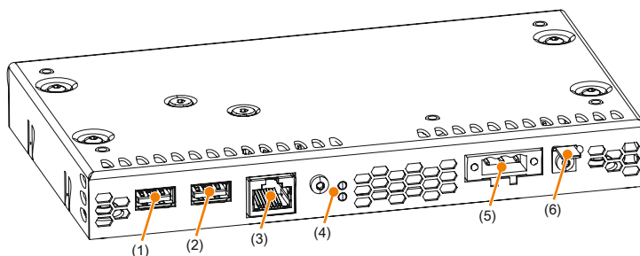
Figure 6: Overview of interfaces - SDL3 receiver link module
