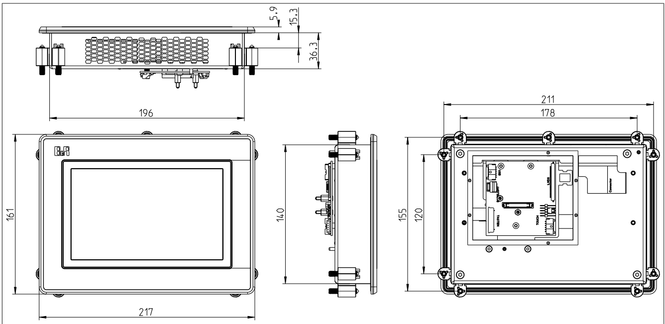
Figure 7: 5AP1120.0702-I00 - Dimensions
