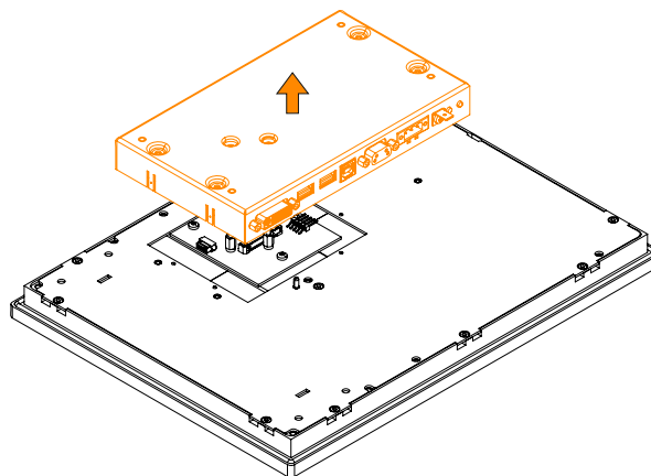
Figure 12: Removing the link module
