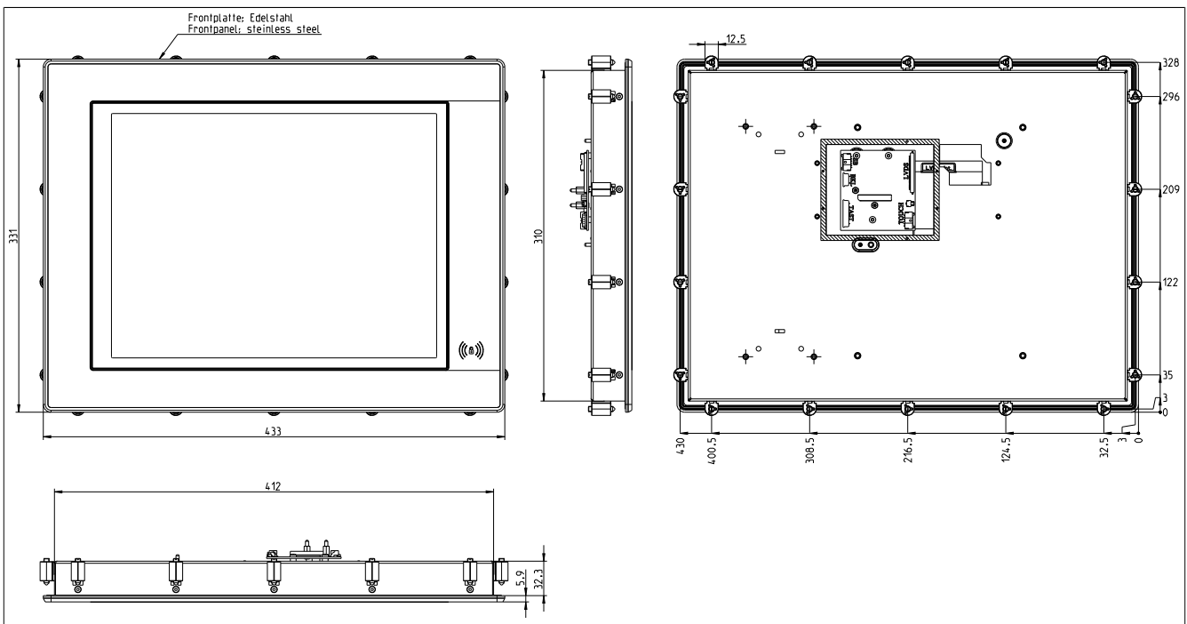
Figure 10: 5AP1125.1505-I00 - Dimensions
