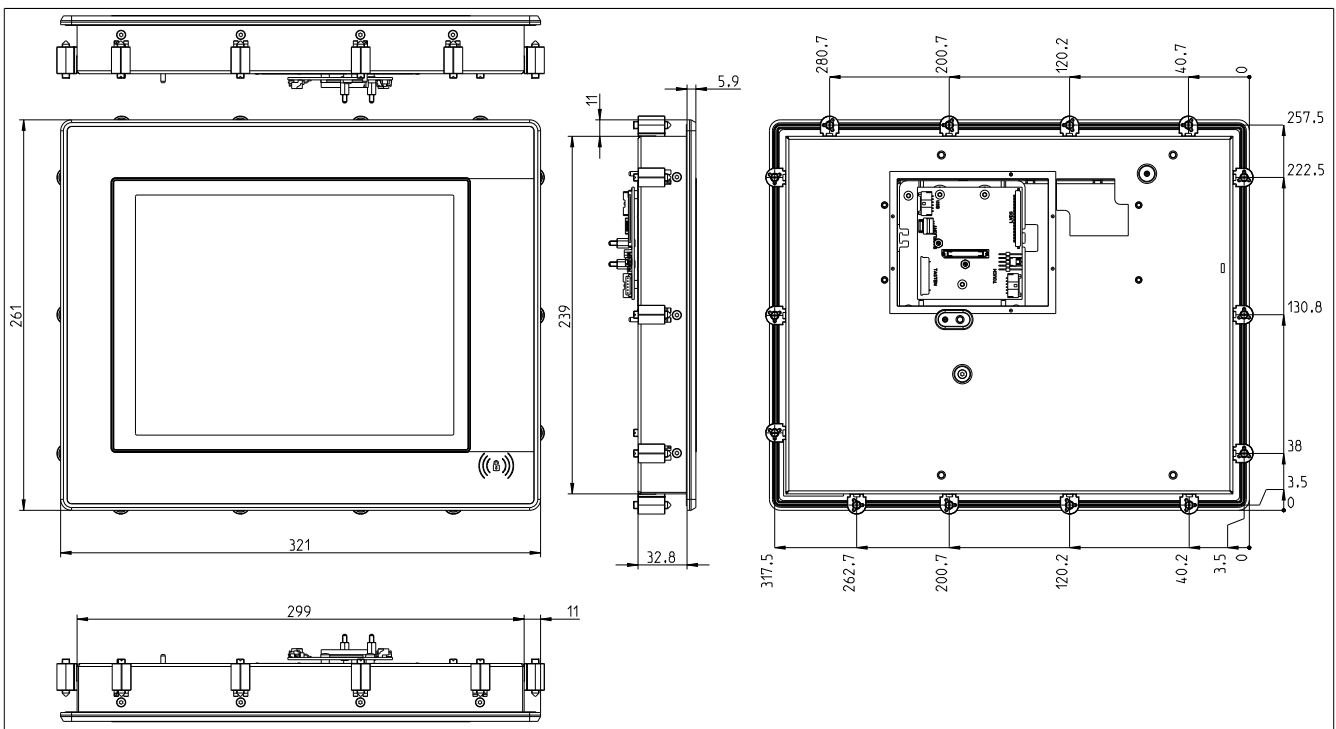
Figure 8: 5AP1125.1043-I00 - Dimensions
